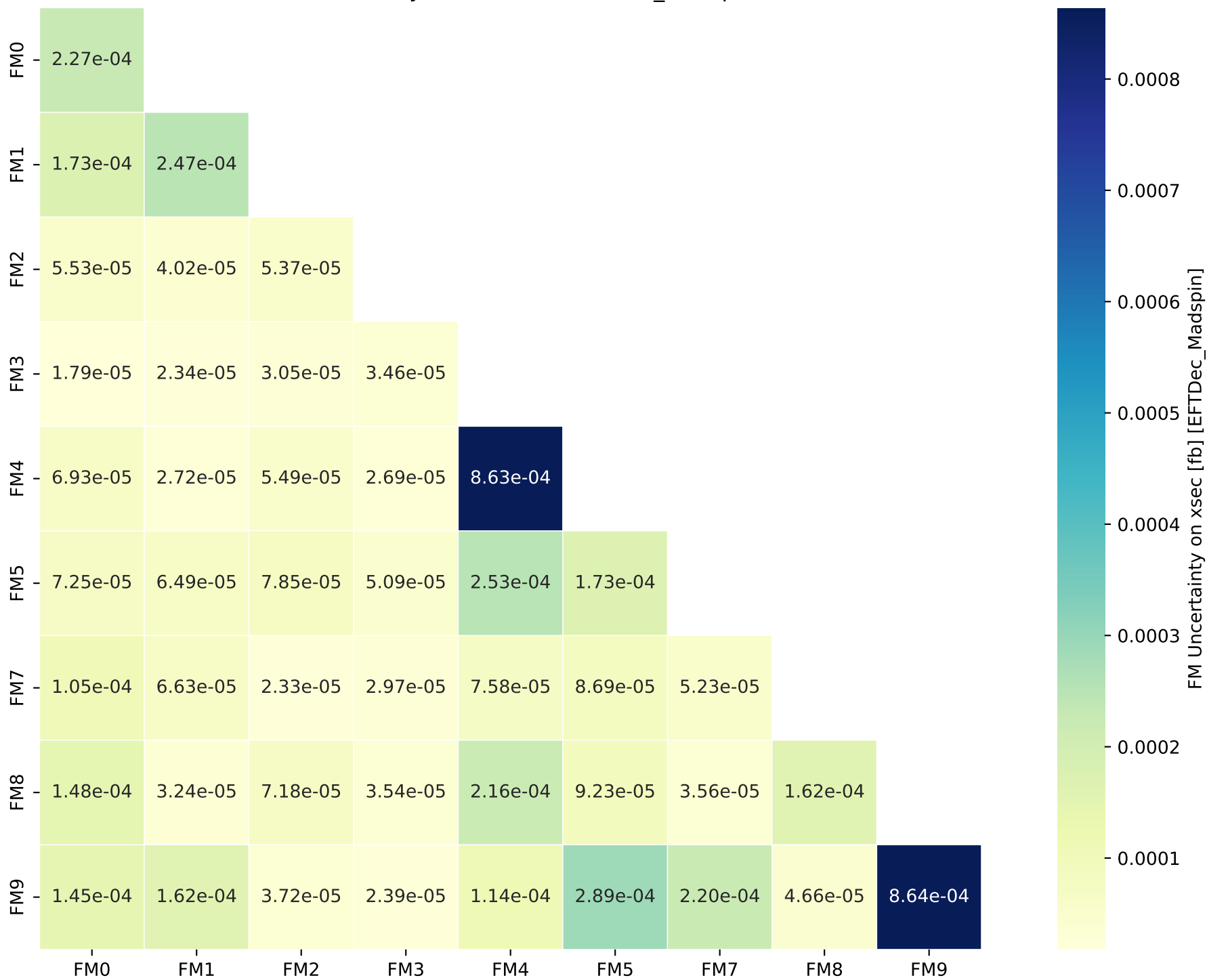
FM Uncertainty on xsec [fb] [EFTDec_Madspin]
